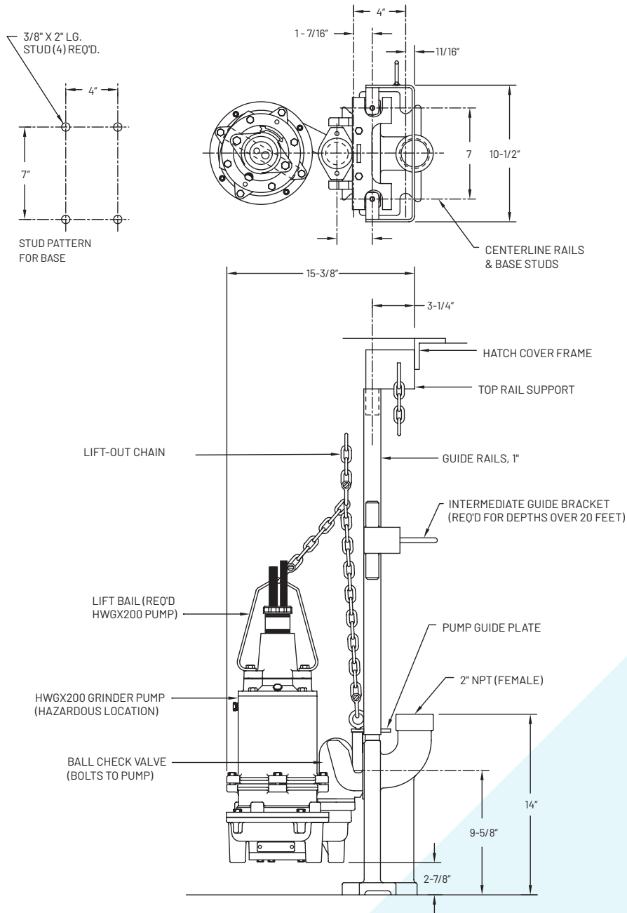
Slide Rail Dimensions (TL-PROX-CV Shown)
