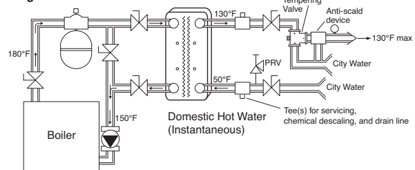
Diagram 3-Instantaneous
