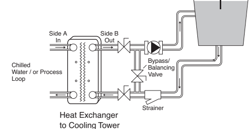
Diagram 3-High Pressure Isolation
