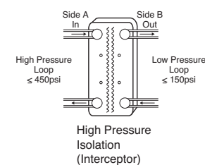
Diagram 3-High Pressure Isolation
